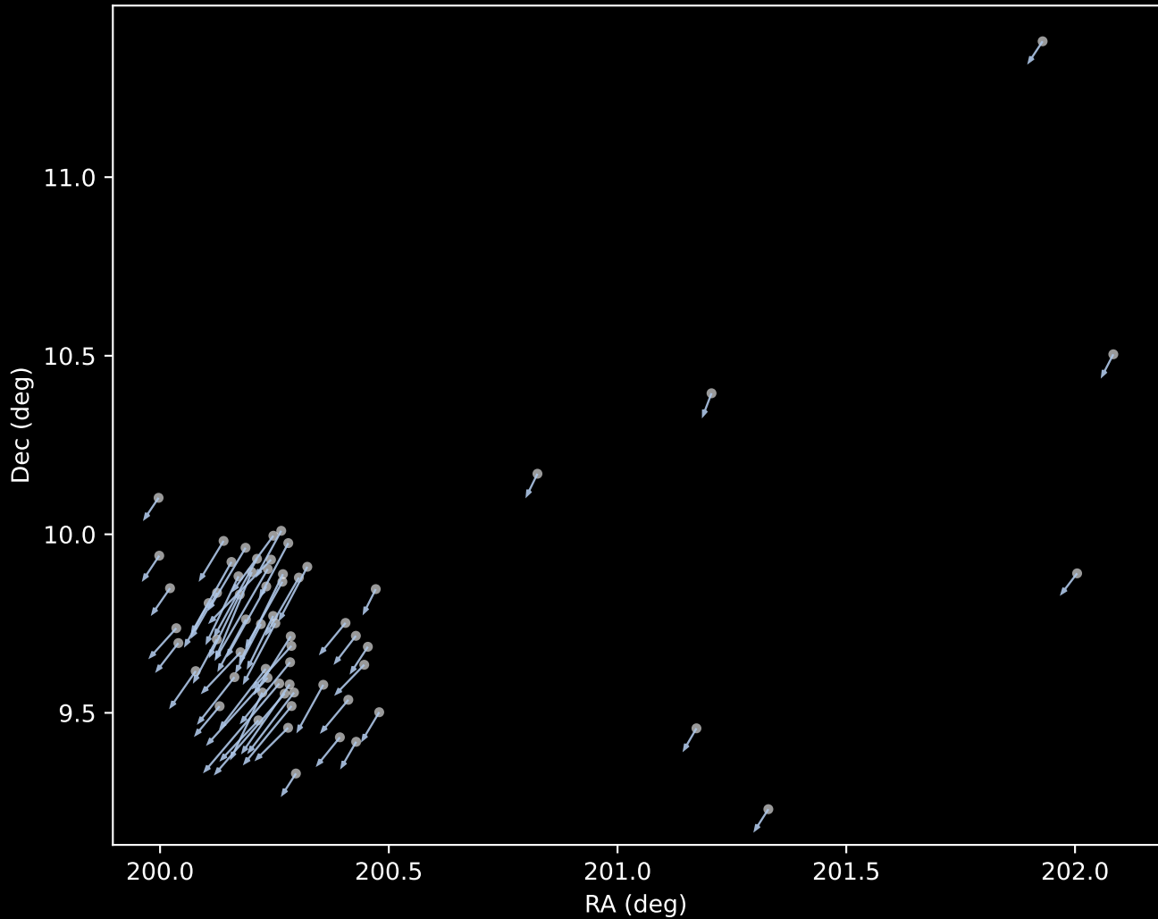
APOGEE DR17 Cluster 1 Proper Motion Vectors (n=64)
