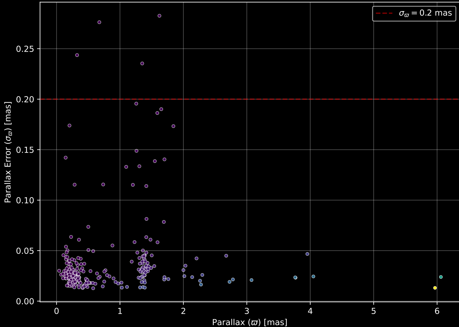
APOGEE DR17 Field: [203+04] Parallax Quality (n= 270)
