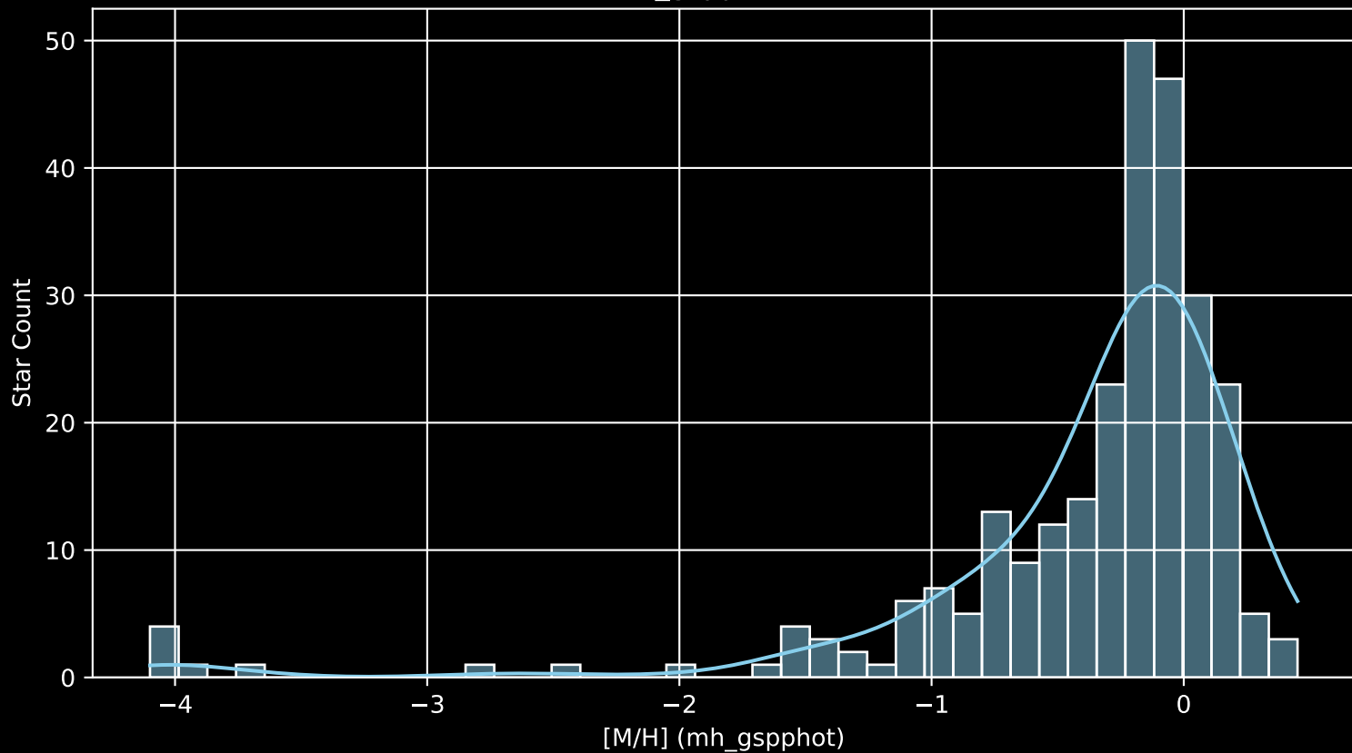
APOGEE DR17 Field: [203+04 [M/H] (mh_gspphot) (n= 267)
