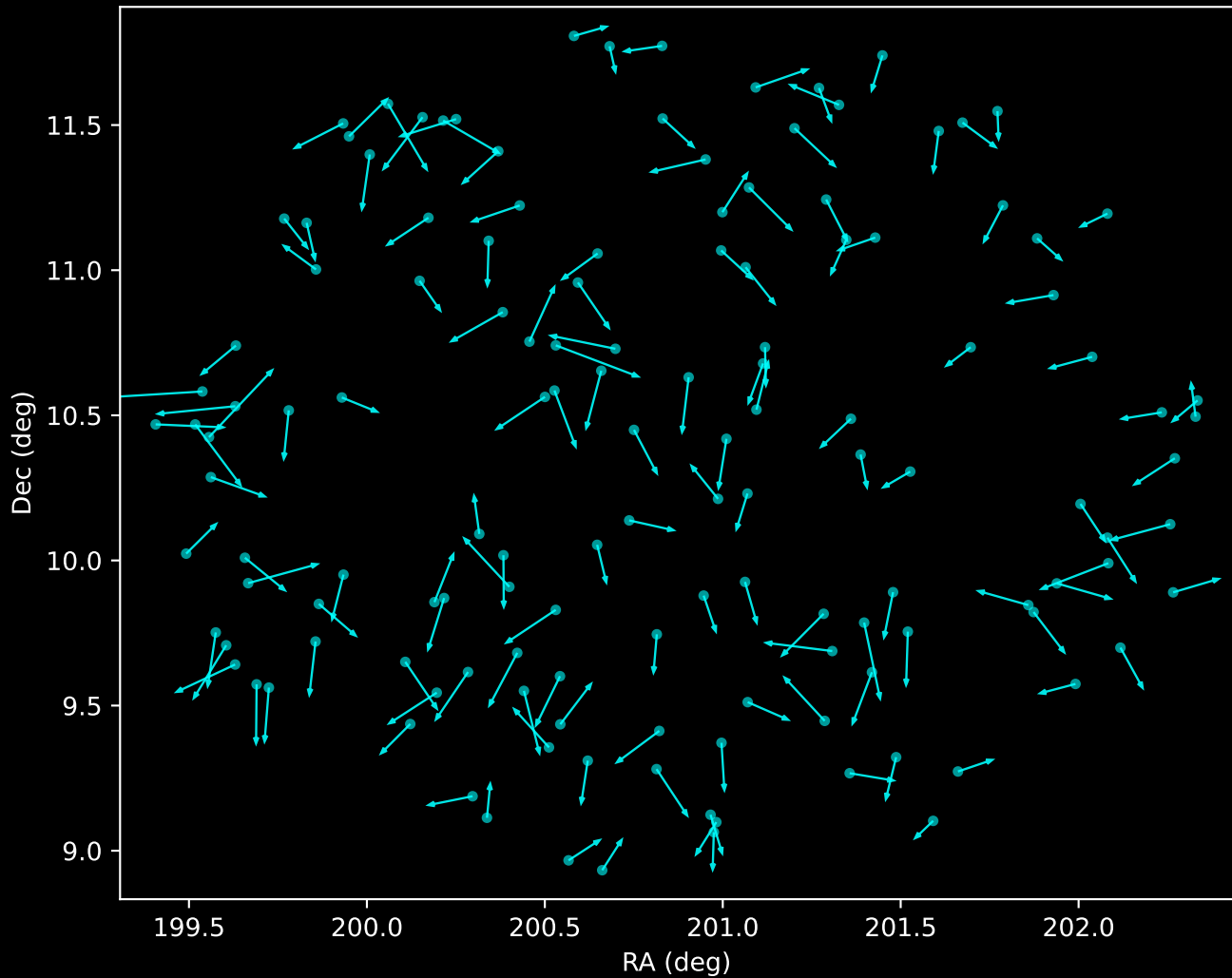
APOGEE DR17 Noise Stream Proper Motion Vectors (n=138)
