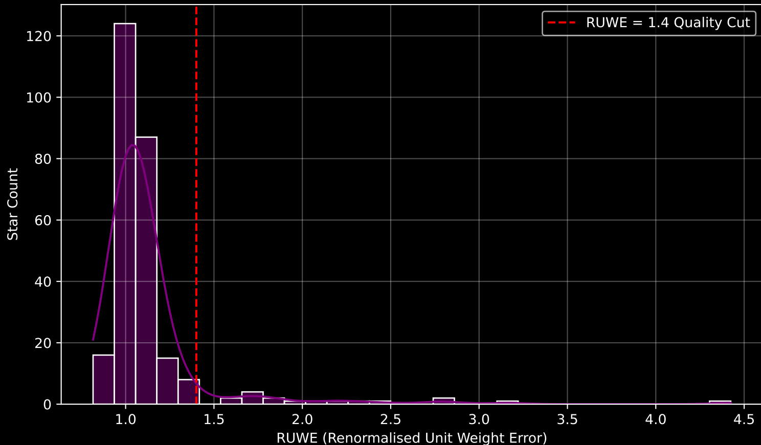
GAPOGEE DR17 Field [203+04] RUWE Distribution (n= 267)
