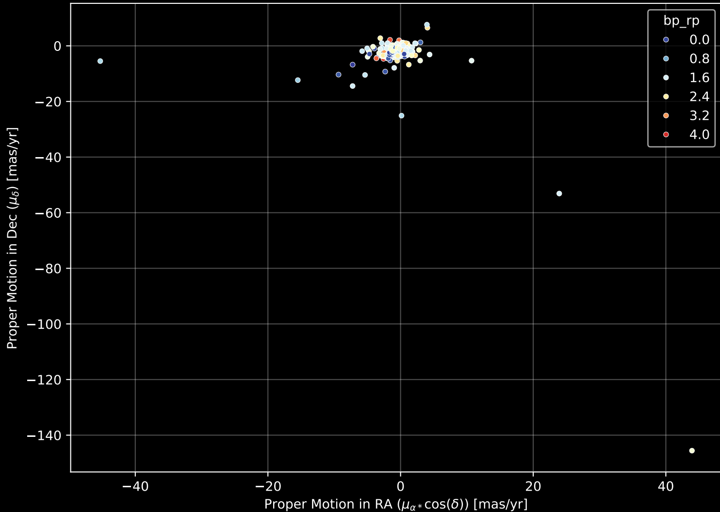
APOGEE DR17 Field: [203+04] Proper Motion Diagram (n= 270)
